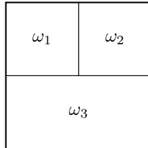
Figure 1: Indirect R-scalability
